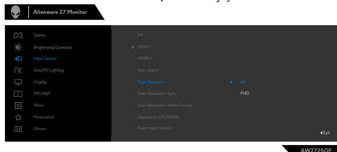
Figure 33. Select Dual-Resolution
