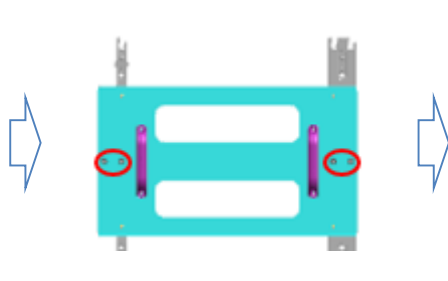
Fig.2 Fixing the Jigs (with screws)
