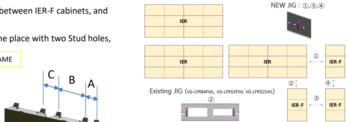
Fig 1. IER-F Extension for General Installation of IER
