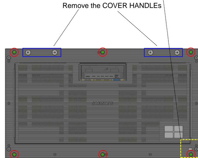
Fig2. Positions to fasten BOLT ETCs when installing the PIVOT
